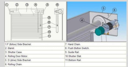
Chain Drive Motor System
