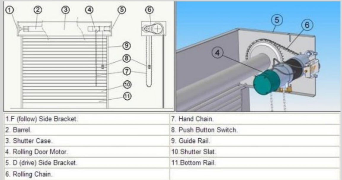
Chain Drive Motor System
