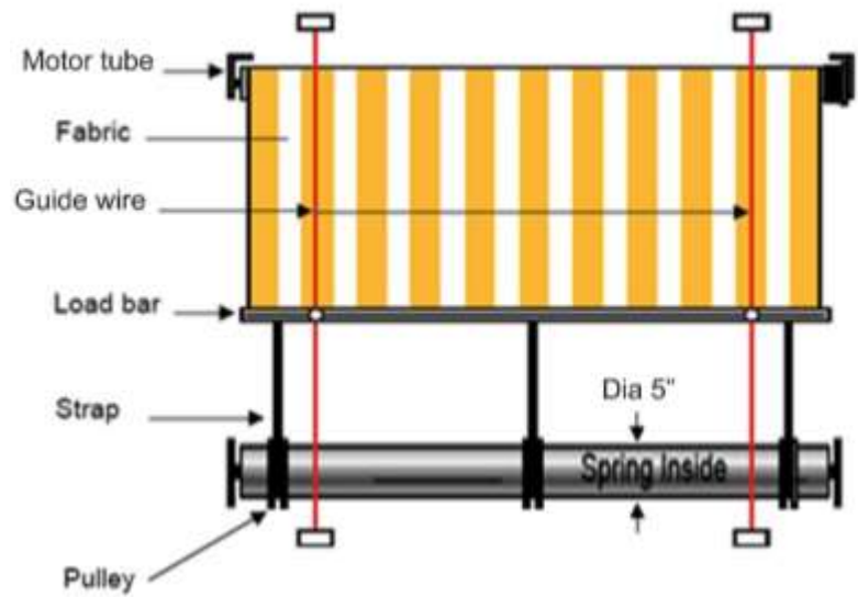
FSS (FABRIC TENSILE SYSTEM SINGLE MOTOR + SRPING)
