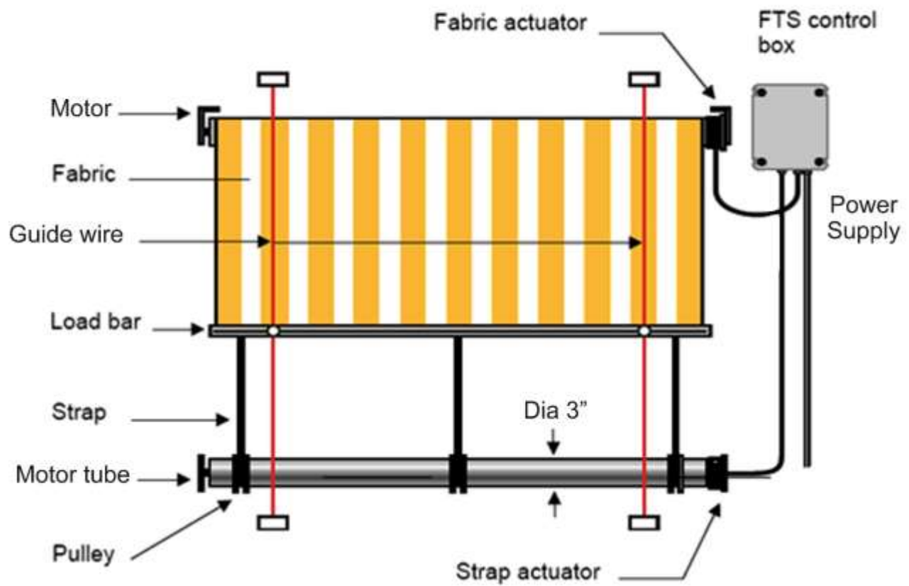
FTS (FABRIC TENSILE SYSTEM DOUBLE MOTOR)
